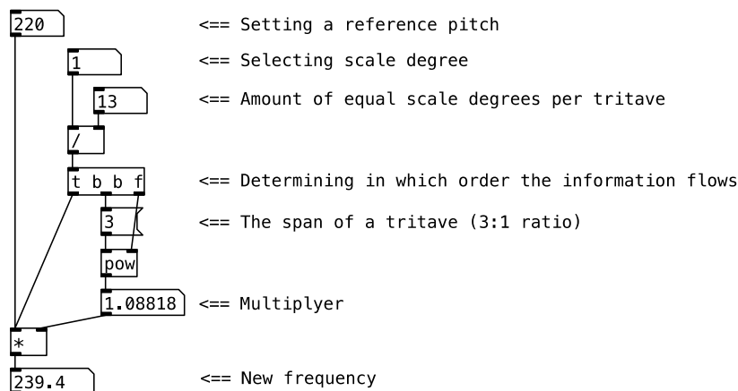
Figure 3: Bohlen-Pierce temperament in Pd.
