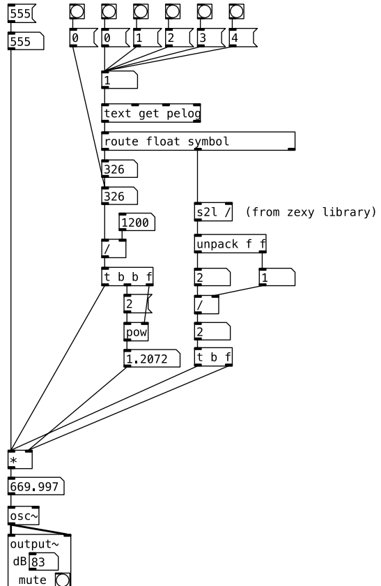
Figure 4: Parsing a Scala file that contains tuning system information with a Pd patch.
